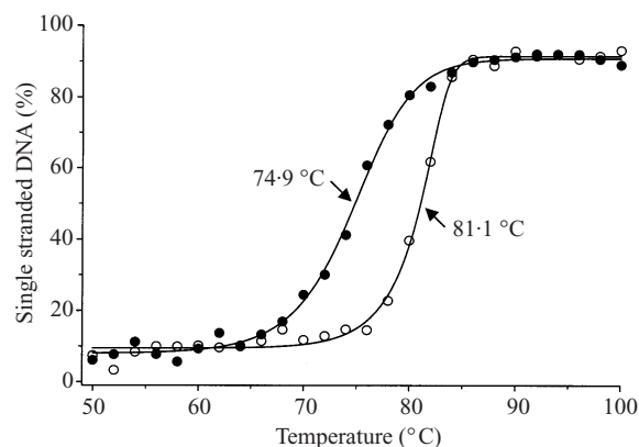
Fig. 1. Melting curves of Solenopsis invicta and Escherichia coli DNA. Open circles represent E. coli and filled circles S. invicta . Each circle represents a mean of two experiments each with two replicates. Arrows indicate melting temperatures.
