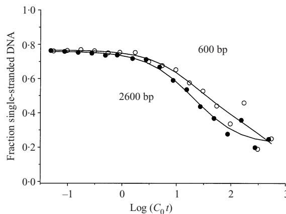
Fig. 2. C_0 t curves for Solenopsis invicta DNA sheared to short and long fragment sizes. Both curves represent the least squares solutions with two components (moderately repetitive and unique sequences). The upper curve (open circles) represents renaturation of short DNA fragments (600 bp) and the lower curve (filled circles) of long DNA fragments (2600 bp). Each circle represents a mean of two experiments each with two replicates.
